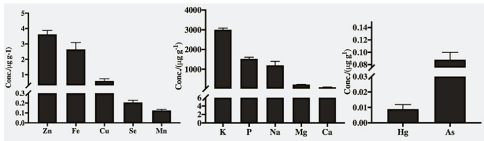
Fig 1. Minerals concentration (µg/g of wet weight) of tilapia fillets from the U.S. marketplace. (a) trace minerals (b) essential minerals (c) heavy
