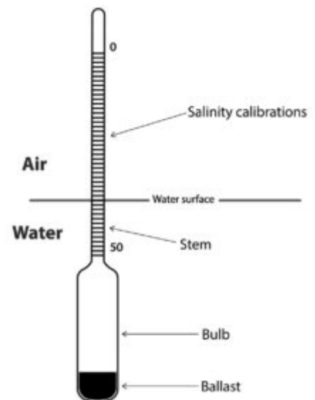
Fig. 2: A density hydrometer.
