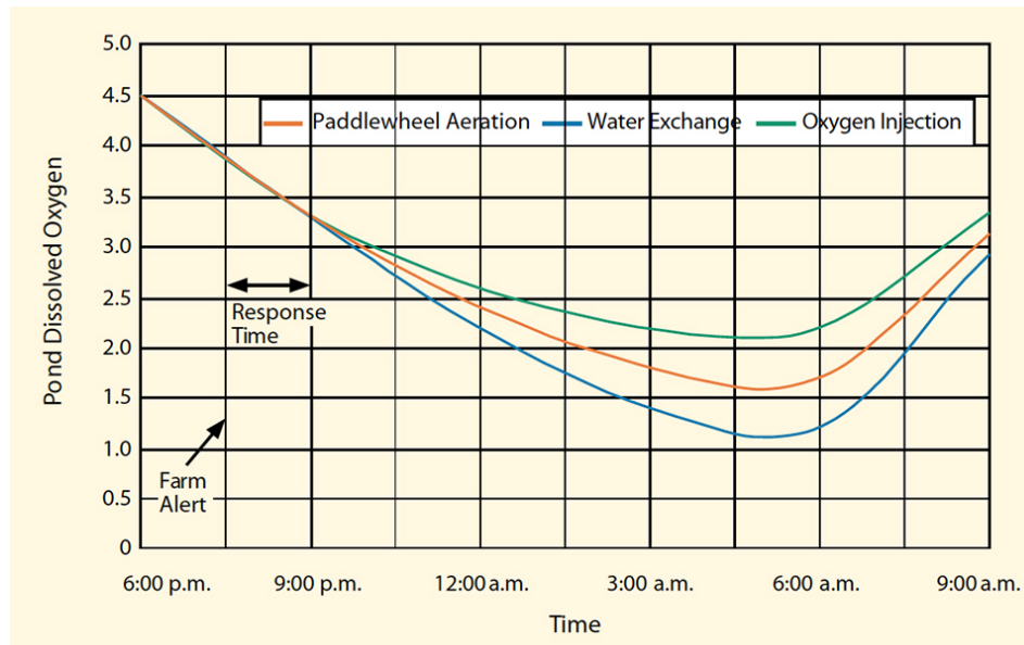
Fig. 1: Based on data collected from various locations in a pond, the above graph shows the effects of emergency aeration systems on rapidly dropping dissolved-oxygen levels.
