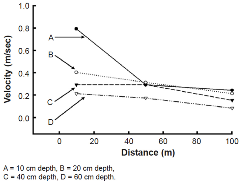
Fig. 3: Water velocity at different distances from a paddlewheel aerator, as measured with an inexpensive, hand-held water current meter.
