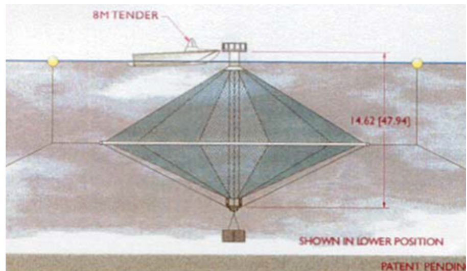
Fig. 2: Sea Station – design and construction.
