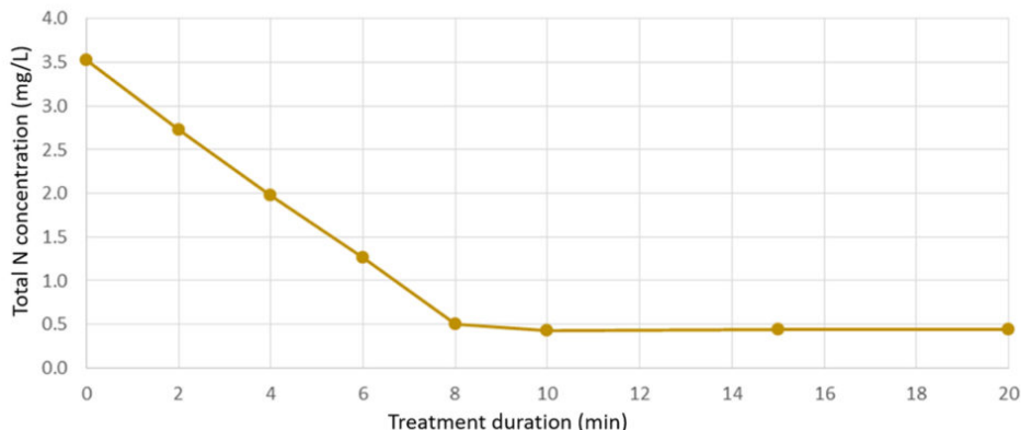
Fig. 2: Concentration of total dissolved nitrogen in the aquaculture water sample spiked with NH4Cl prior to electrochemical treatment. Volume was 1000 mL; anode = BDD; cathode = Copper; applied with 5 Volts.
